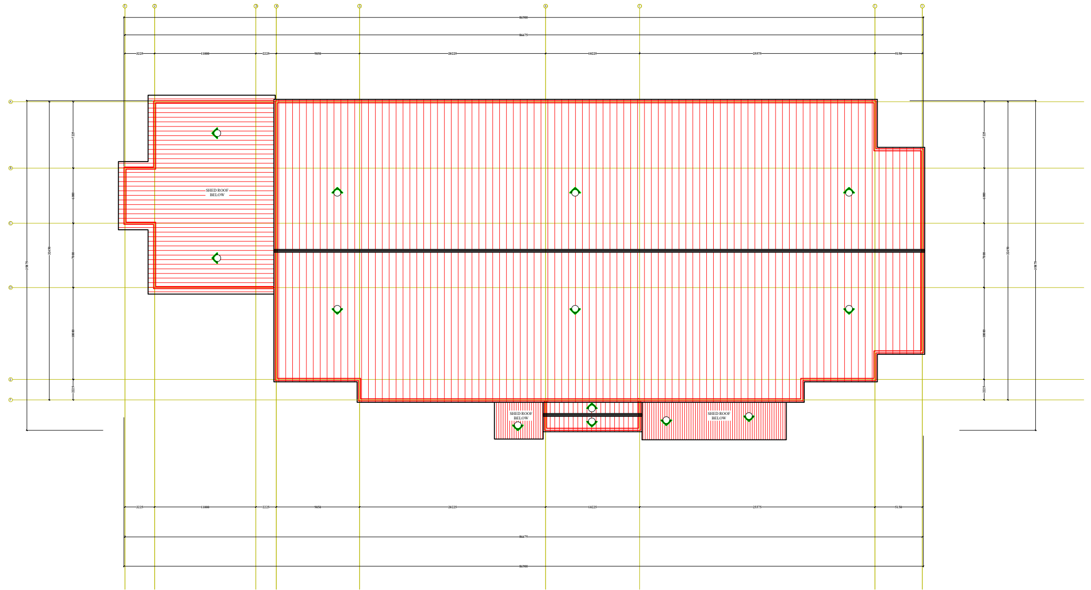
ROOF PLAN
