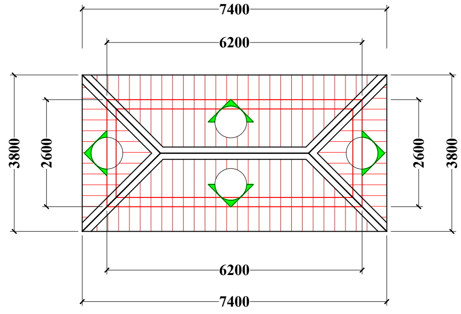
ROOF PLAN
